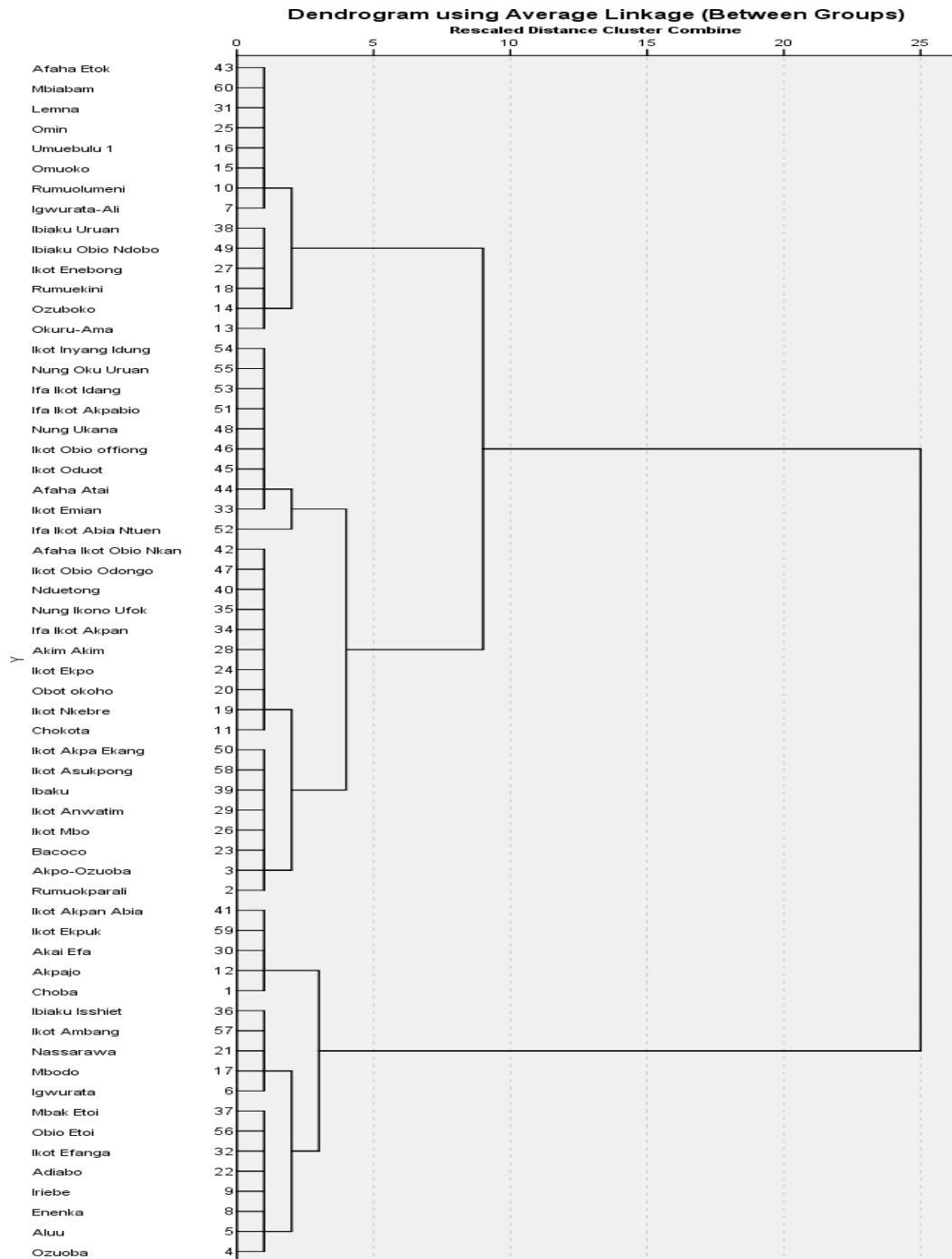
Dendrogram Using Average Linkage (Between Groups)
